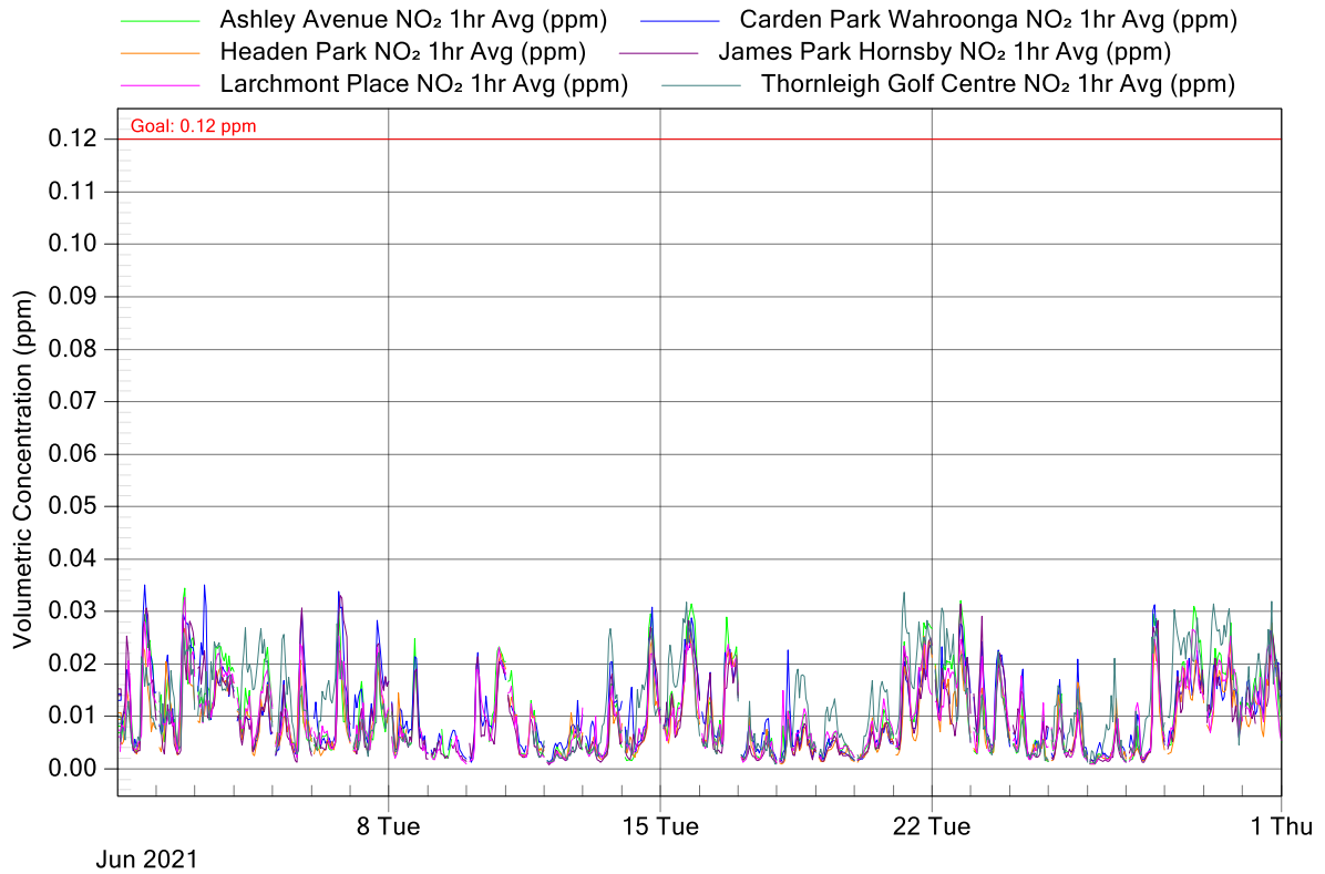
Figure 3: NorthConnex Project Air Monitoring Stations - NO 2 1 Hour Averages for June 2021
