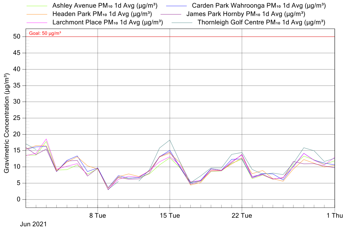
Figure 4: NorthConnex Project Air Monitoring Stations - PM 10 1 Day Averages for June 2021
