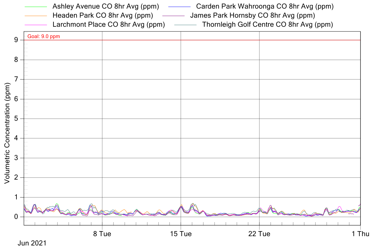
Figure 2: NorthConnex Project Air Monitoring Stations - CO 8 Hour Rolling Averages for June 2021
