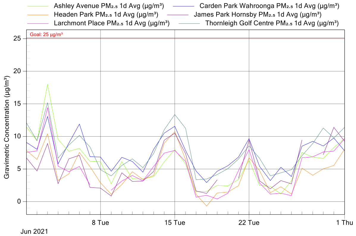
Figure 5: NorthConnex Project Air Monitoring Stations - PM 2.5 1 Day Averages for June 2021
